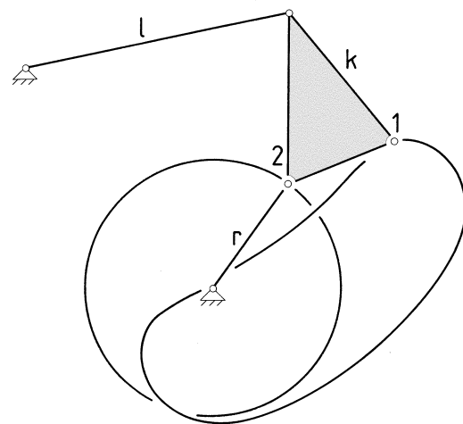
Figure 1. Scheme of a three-bar linkage
