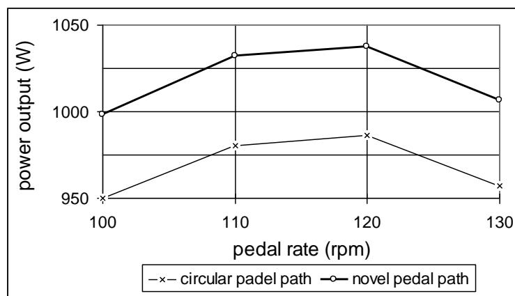
Figure 2. Maximal power output (averaged) on the circular pedal path and the novel pedal path [1]
